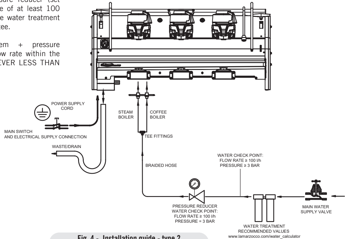
Fig. 4 - Installation guide - type 2
