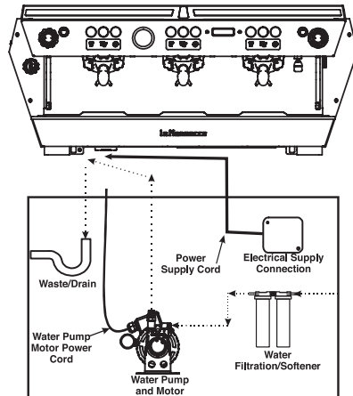
Fig. 2 - Installation Guide
