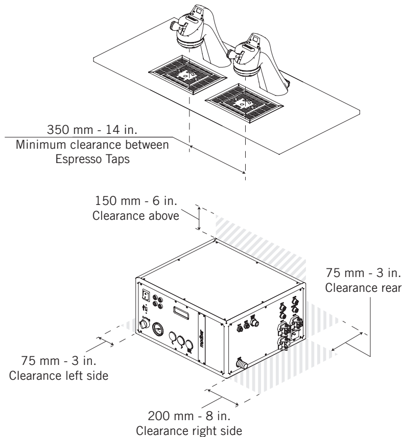
Fig. 2 - Installation guide
