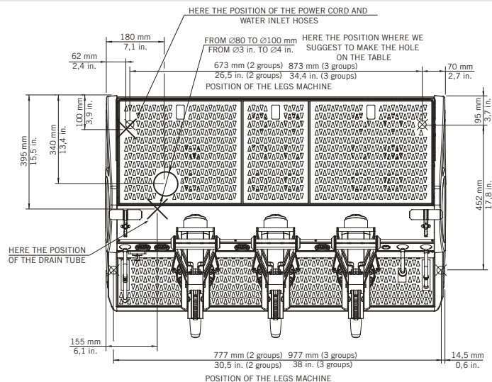
Fig. 3 - Installation guide
