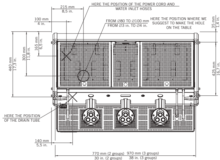
Fig. 2 - Installation guide
